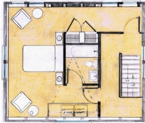
Plan 1 – SECOND FLOOR
